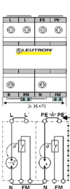
two-pol. bus-bar connection
